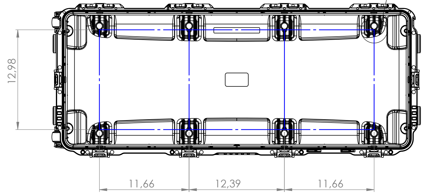
BASE SCREW BOSS PATTERN
