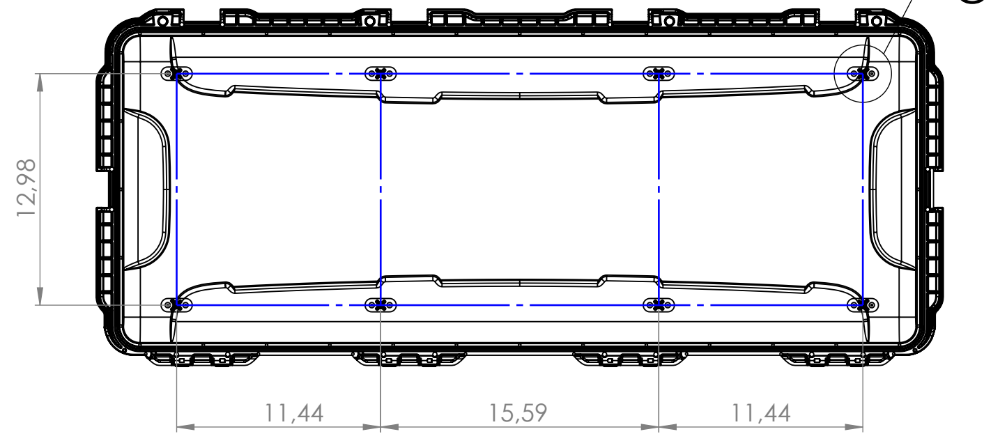
LID SCREW BOSS PATTERN
