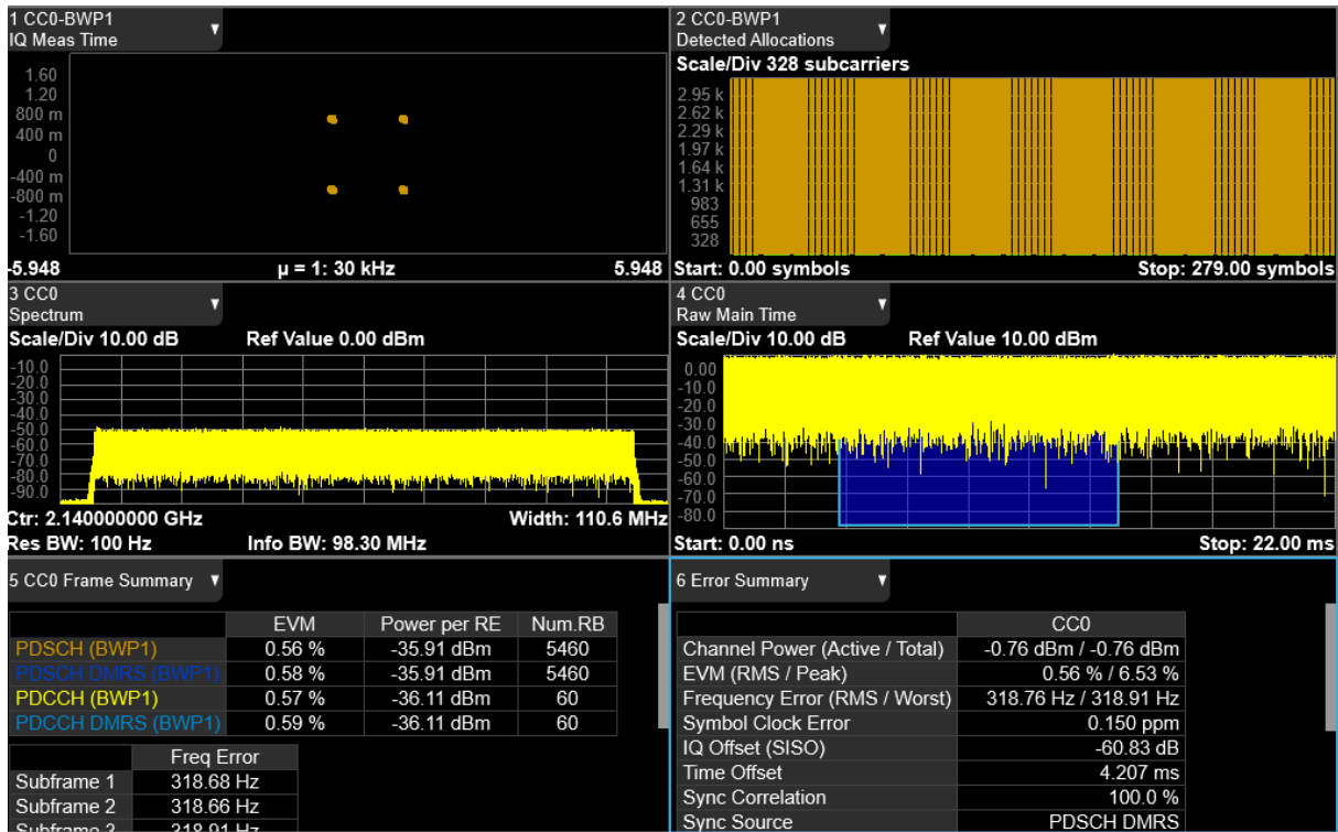
5G NR Test Mode TM1.1 100M Bandwidth 3.9G Carrier, EVM Test Value
