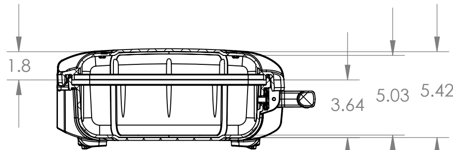
SECTION B-B
