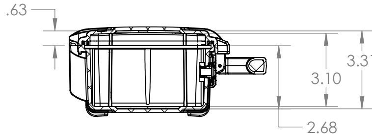
SECTION B-B
